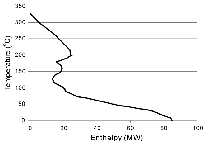
Fig. 4. Grand composite curve for the RCU, \Delta T_{min} = 45 °C.
