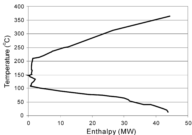
Fig. 3. Grand composite curve for the CDU average feed case, \Delta T_{min} = 30 °C.
